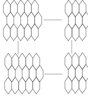
Figure 3. Graphene G_{t,s}
