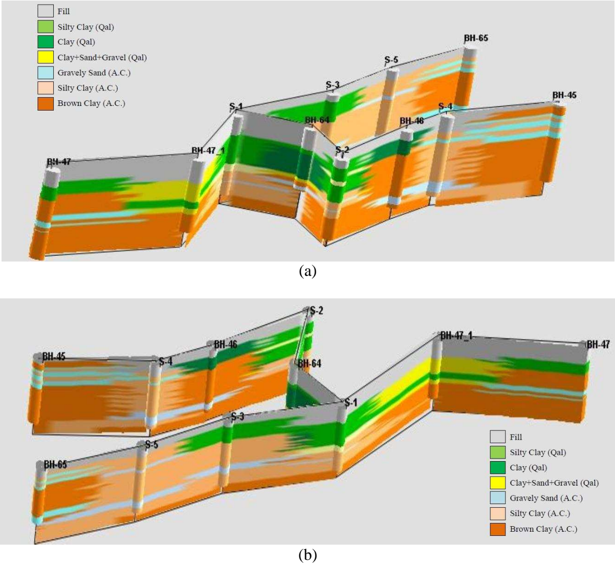
Figure 12. Regional 3D subsurface panel diagram created by interpreting 2D electrical resistivity images and borehole logs together a) North to South, b) South to North [10].
