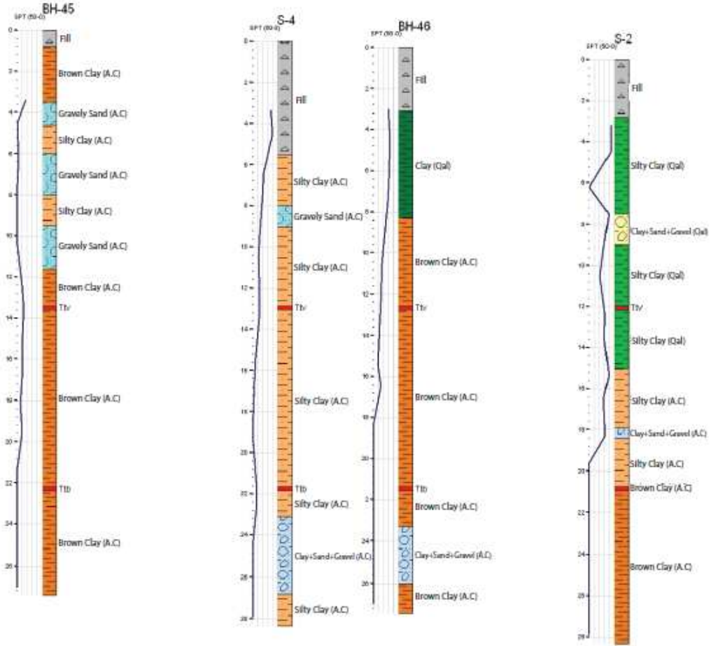
Figure 3. Line 1 boring logs.
