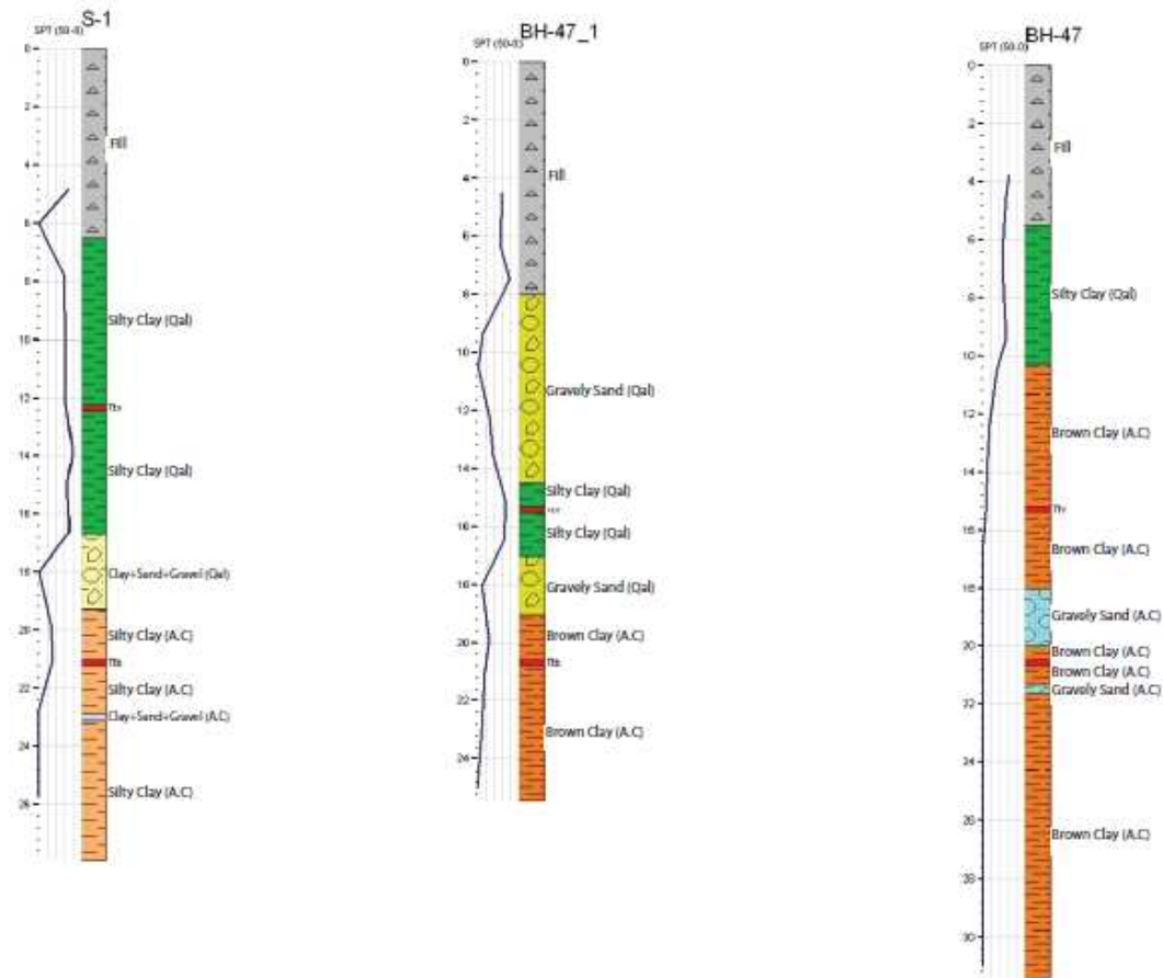
Figure 7. Line 2 boring logs (cont'd).
