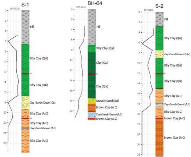
Figure 4. Boring logs between Line1 and Line 2.
