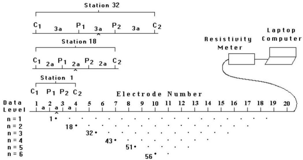
Figure 8. The arrangement of electrodes for a 2-D electrical survey and the sequence of measurements used to build up a pseudosection [3].
