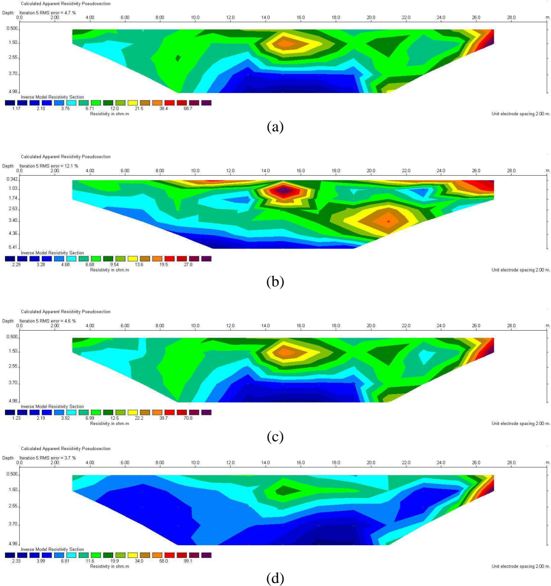
Figure 9. Interpretation of a) Schlumberger N6 Dipole Dipole N4, b) Dipole Dipole N6S1, c) Schlumberger N6, d) Wenner Alpha electrode configurations for profile 1 [10].
