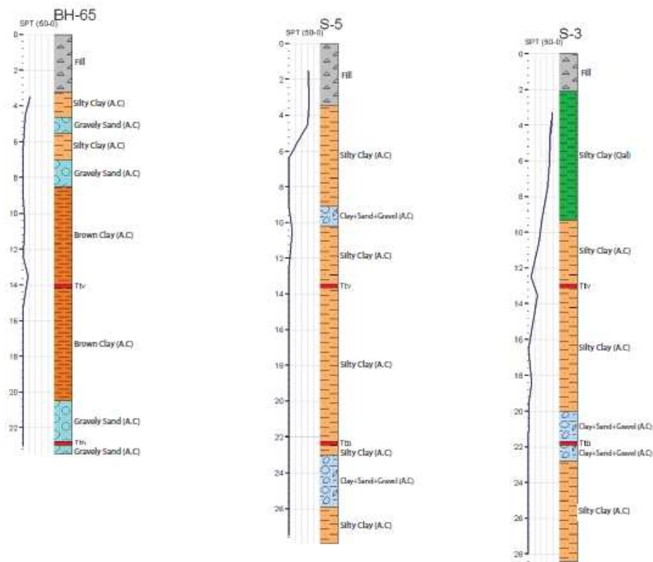
Figure 5. Line 2 boring logs.
