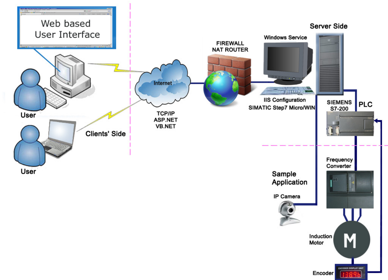
Figure 1. General Architecture of the designed system by asynchronous motor speed control with frequency convertor experiment.
