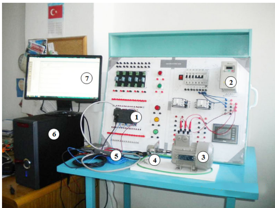
Figure 5. General view of the Designed web based remote access PLC training set.
