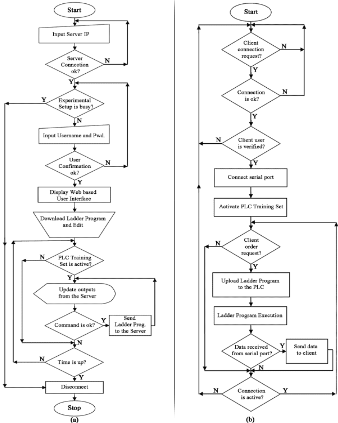
Figure 3. (a) Client and (b) Server software flow chart of the Designed System
