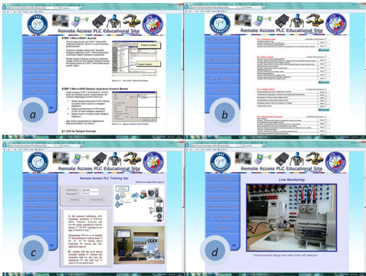
Figure 6: Web user interfaces samples of Remote Access PLC Web Site
