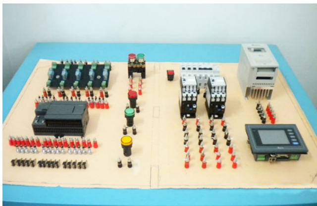
Figure 4. A view of the experiment set from the design phase
