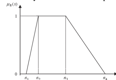
Figure 1. Trapezoidal fuzzy number \tilde{n}
