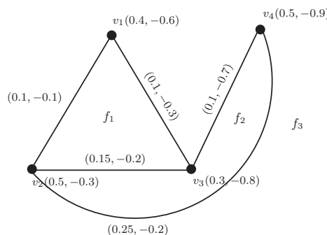
FIGURE 4. Faces in PBFPG.
