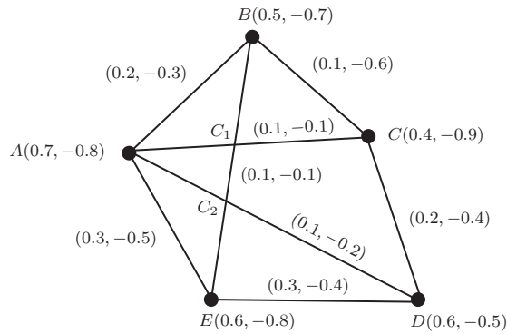
FIGURE 6. PBFPG of a road network.
