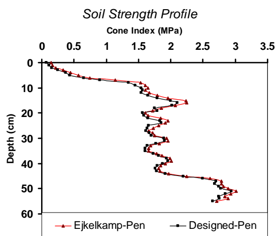
Fig. 3. Average soil strength profile for the hand-pushed penetrometers
