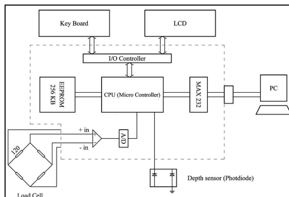
Fig. 2. Block Diagram of the Data Logging System
