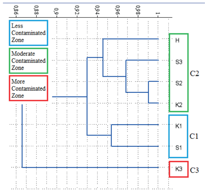
Figure 2. CA diagram.
