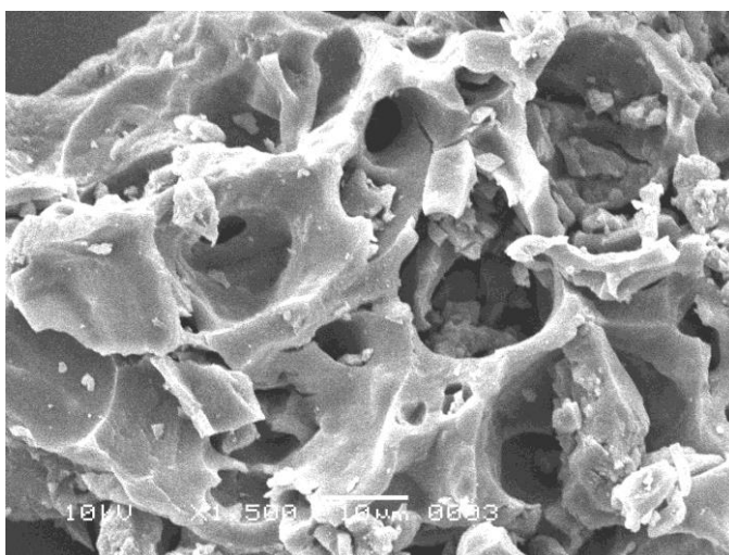
Figure 2. SEM image of activated carbon prepared from corn husk
