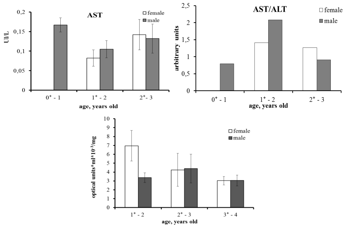
Figure 5. Age-dependent changes of aminotransferase activities in the liver of T. mediterraneus .
