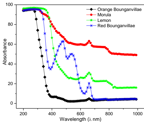
Fig. 3. Absorbance spectra of four natural dyes prepared on glass substrates
