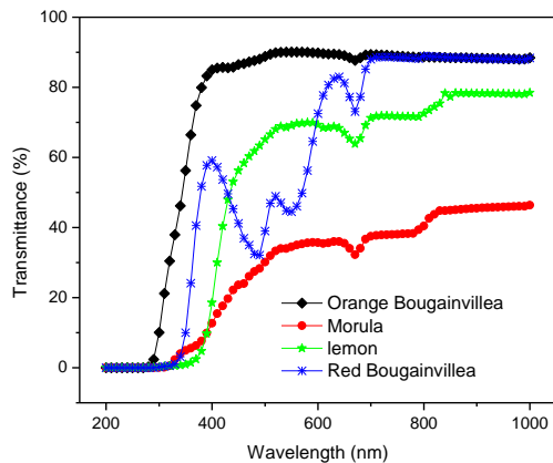
Fig. 2. Transmittance spectra of four natural dyes prepared on glass substrates
