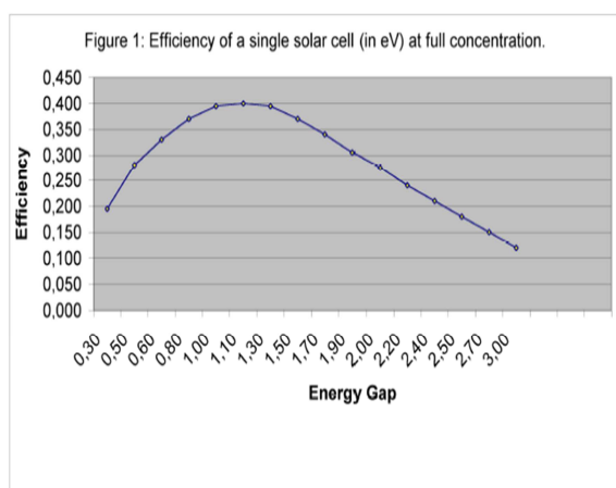
Fig. 1. Efficiency of a single solar cell (in eV) at full concentration.
