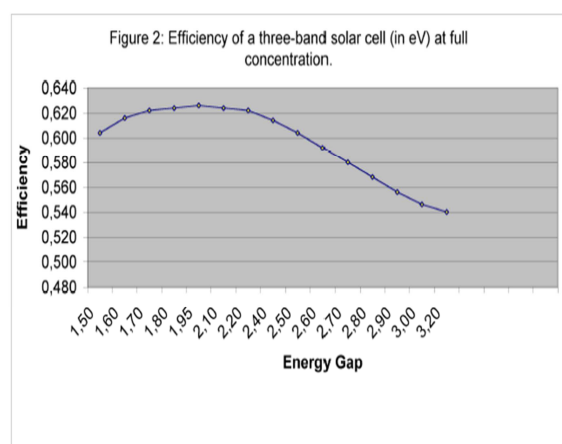
Fig. 2. Efficiency of a three-band solar cell (in eV) at full concentration.
