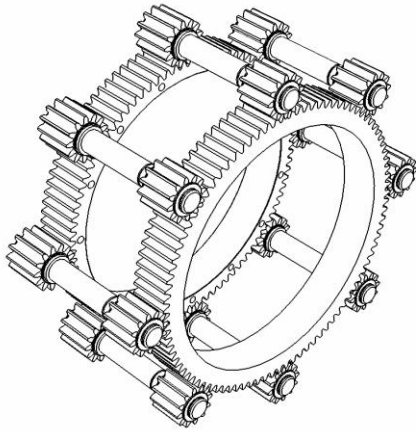
Fig.14. Two-stage planetary gear system
