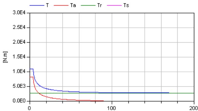
Fig.1. Torque-behaviour of the drive
