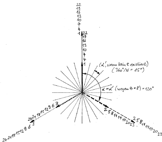
Fig.9. Phase angles of the electromagnetic force of the wires in neighbored nuts
