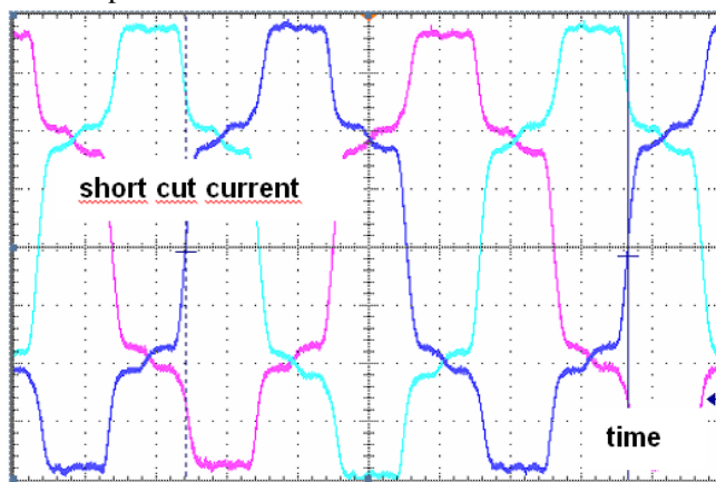
Fig.13. Qualitative diagram of the short cut current of the three phases
