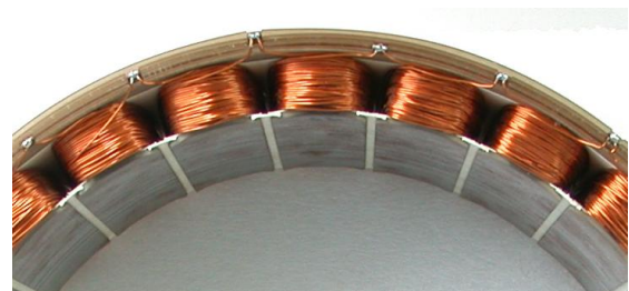
Fig.8. 3phase single tooth winding of the electric machine
