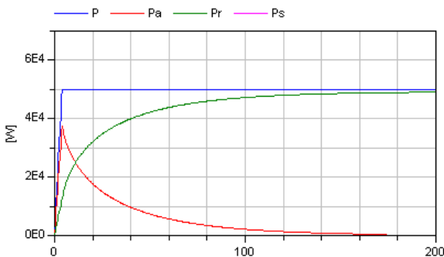
Fig.2. Power-behaviour of the drive
