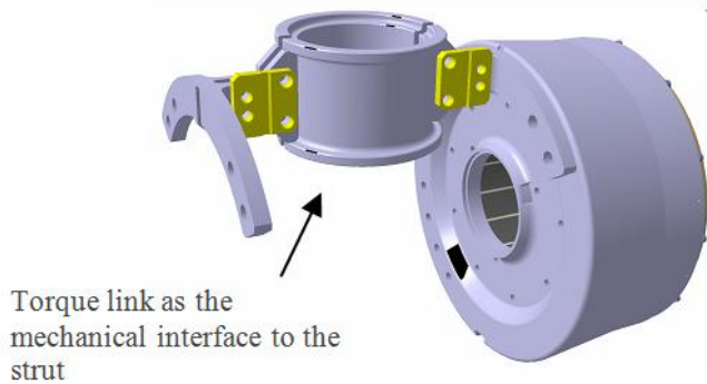
Fig.6. Torque link as the mechanical interface to the strut of the nose leg gear
