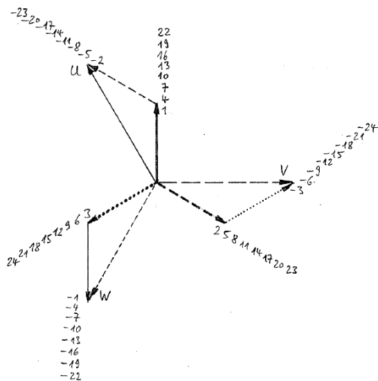
Fig.10. Combination of the electromagnetic forces of the wires in neighbored nuts to the 24 coils of the three phase winding
