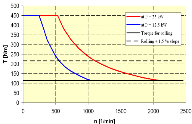
Fig.7. Torque-speed behaviour of one electric machine
