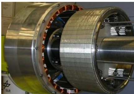
Fig.16. Rotor of the electric machine which carries the permanent magnets and the planet gears
