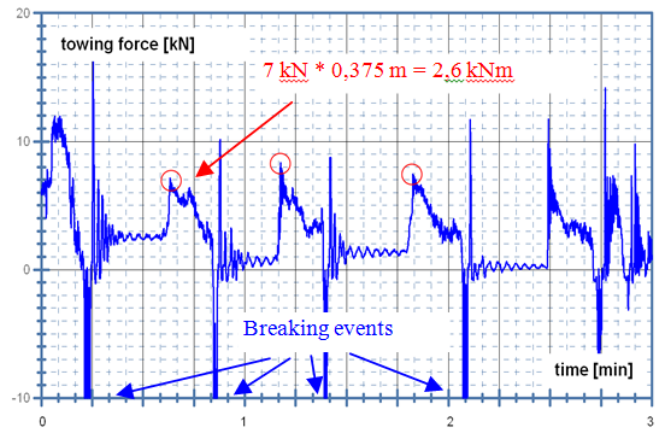
Fig.4. Towing force measurement of an aircraft Airbus A319
