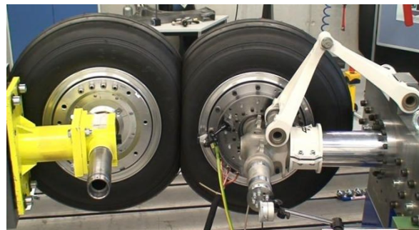
Fig.18. Static load test of the drive by pressing a driven wheel against a freely mounted wheel
