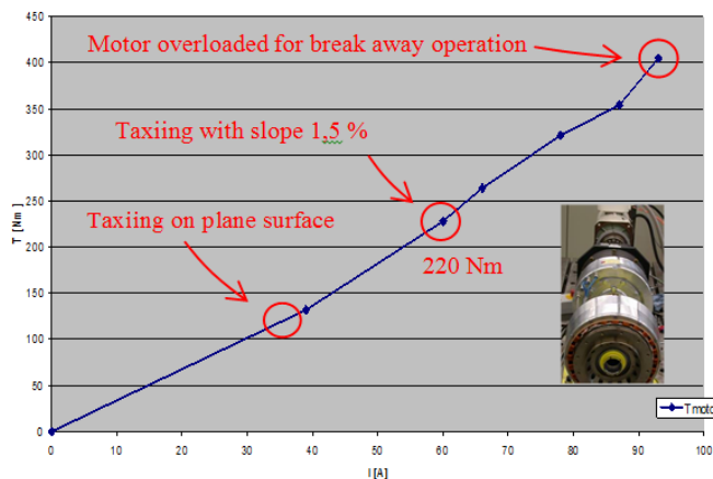
Fig.20. Torque of a single electric machine
