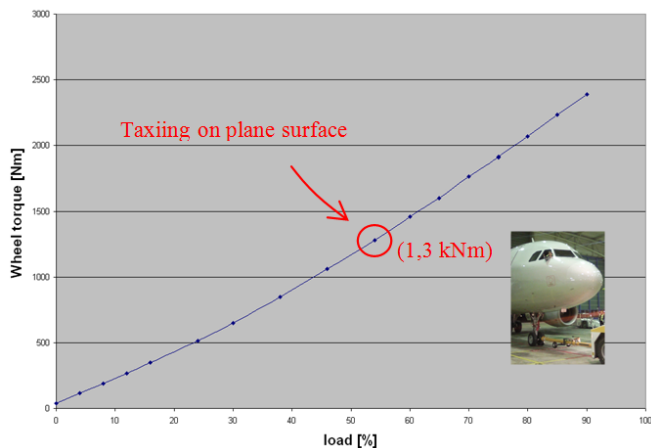
Fig.19. Torque at the rim of one wheel
