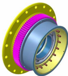
Fig.15. Stator-sided parts of the gear and the clutch, called the intermediate shaft
