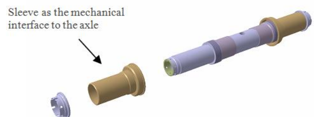
Fig.5. Sleeve as the mechanical interface to the axle of the nose leg gear
