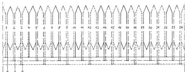
Fig.11. Winding diagram of the three phase winding with 24 nuts and 24 coils, consisting of 8 parallel delta-connected systems
