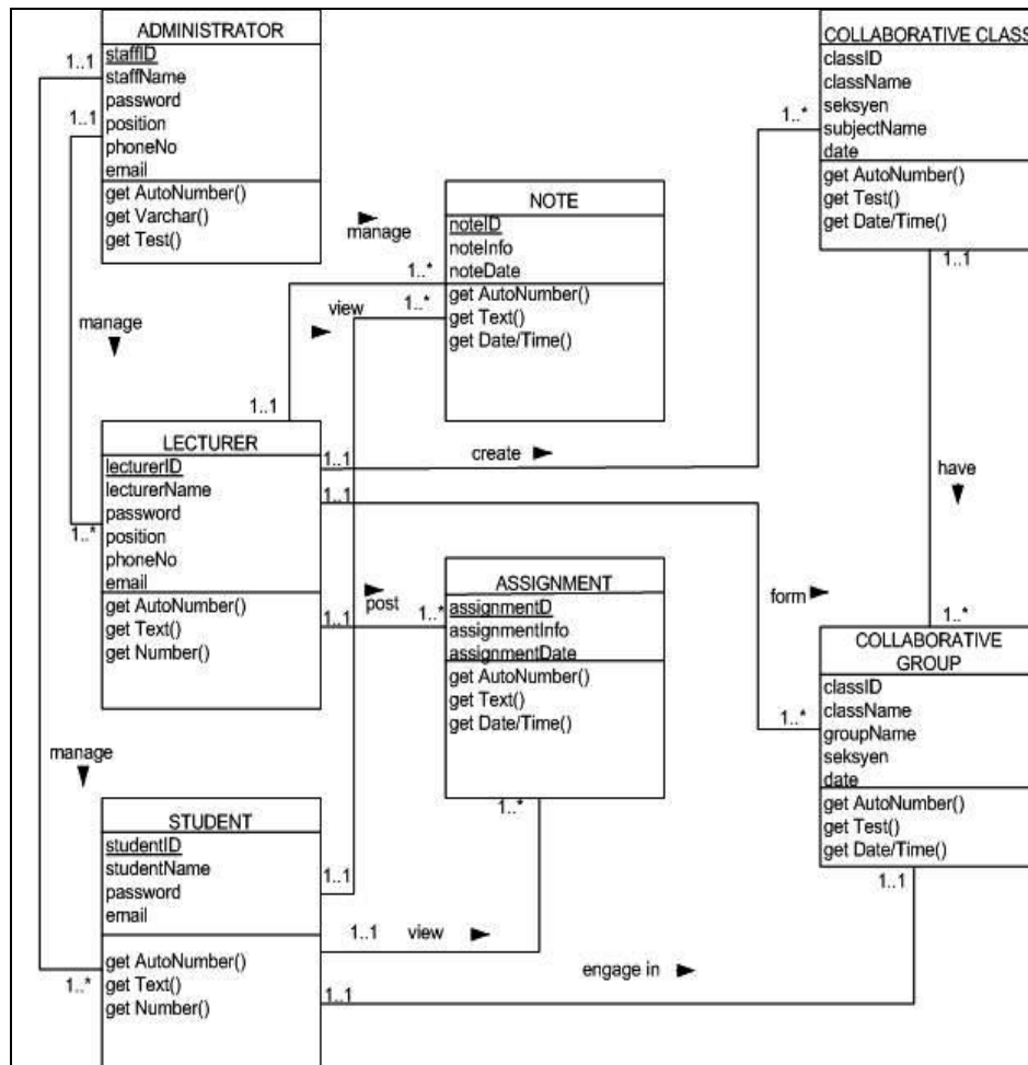
Figure: 3 Class Diagram for OCLS
