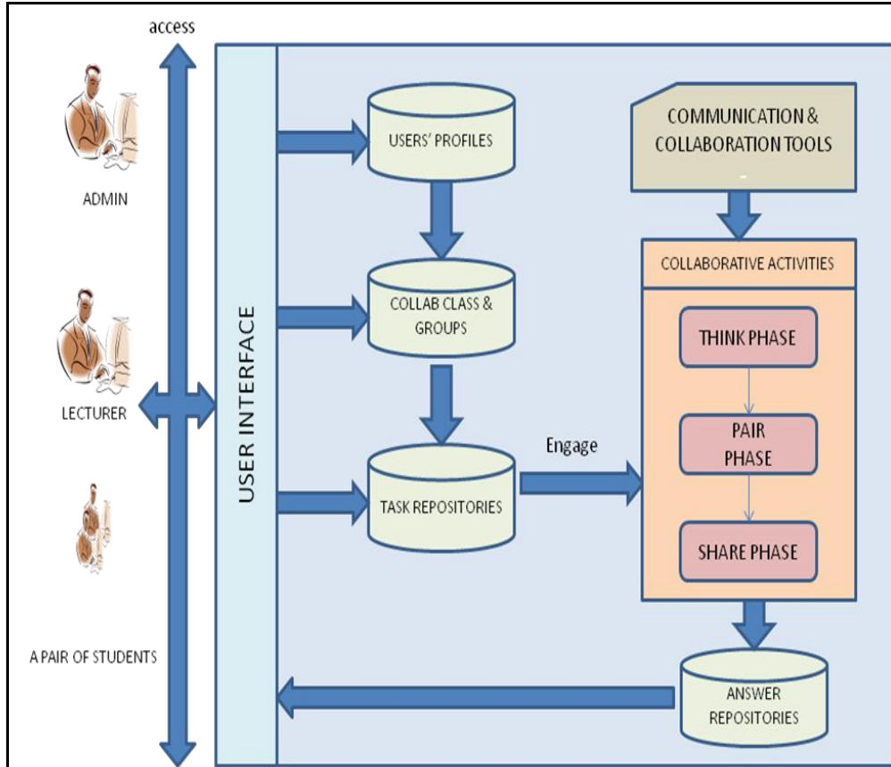
Figure: 4 Proposed model of system's architecture for OCLS
