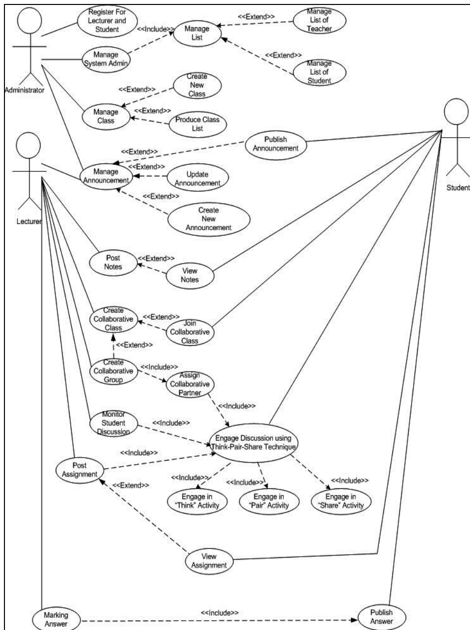
Figure: 2 Use-Case diagram for OCLS
