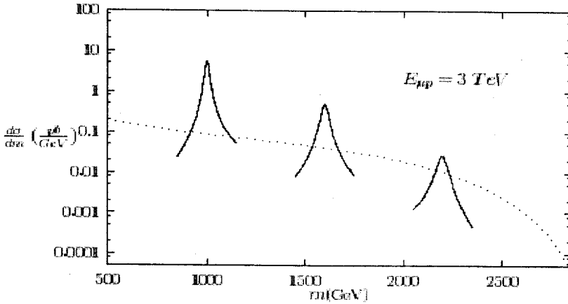
Figure 3. At \mu p collider, invariant mass distribution \mu p \rightarrow ljX . Resonance peaks are shown for M_{\mu g} = 1000, 1600 and 2200 GeV, respectively. Dotted line denotes the SM backgrounds.
