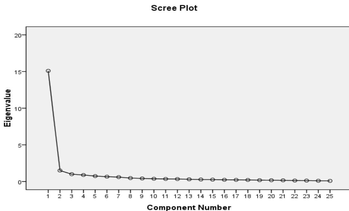
Figure 2. Eigenvalue-Factor structure
