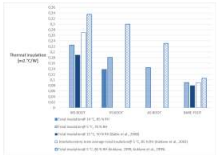
FIGURE 3 TOTAL THERMAL INSULATION RESULTS FOR THE THREE BOOT MODELS, TESTED IN TWO ENVIRONMENTAL CONDITIONS: A COMPARISON IS CARRIED OUT WITH THE INTERLABORATORY TESTS, BABIC TESTS AND KUKLANE TESTS.
