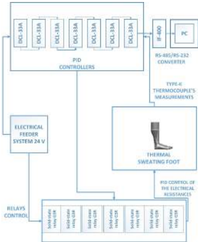
FIGURE 2 BLOC DIAGRAM OF THE HEATING SYSTEM.
