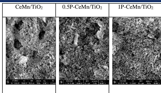
Fig. 3. SEM images of CeMn/TiO 2 , 0.5P-CeMn/TiO 2 and 1P-CeMn/TiO 2 catalysts
