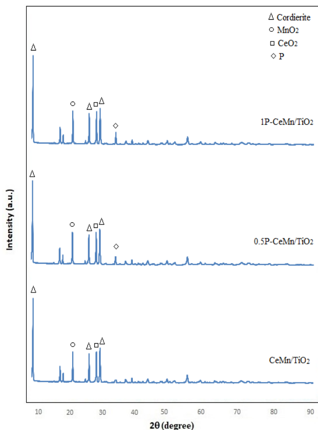
Fig. 5. XRD patterns of CeMn/TiO 2 , 0.5P-CeMn/TiO 2 and 1P-CeMn/TiO 2 catalysts
