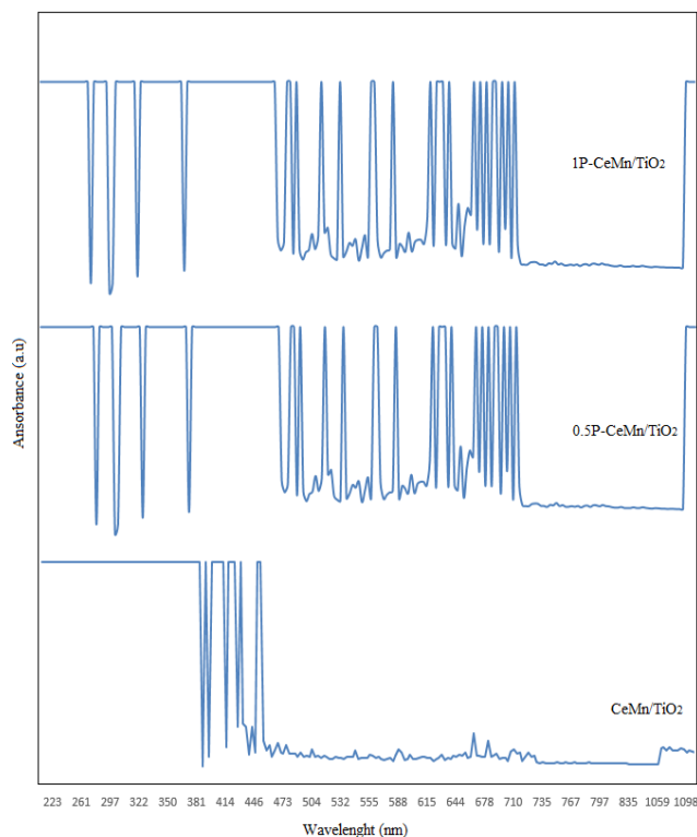
Fig. 6. UV-Vis spectra of CeMn/TiO 2 , 0.5P-CeMn/TiO 2 and 1P-CeMn/TiO 2 catalysts
