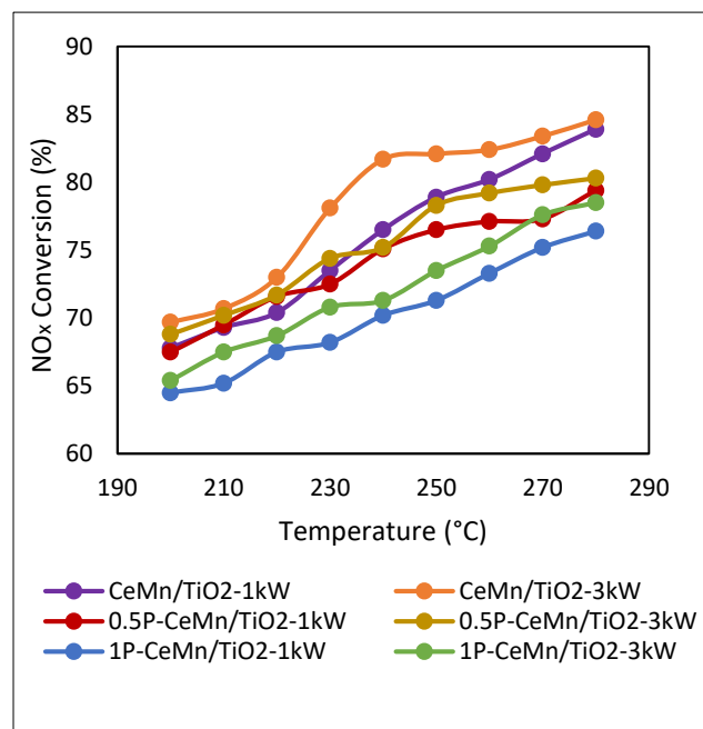
Fig. 2. NO x conversions of catalysts at 1 kW and 3 kW engine loads
