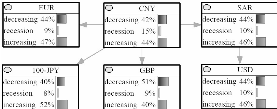
Figure 7. DAG model of Scenario-D with Evidence values
