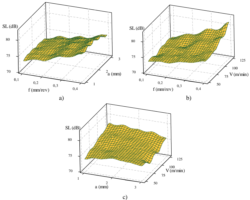
Figure 8. Sound level versus a) feed rate and depth of cut, b) feed rate and cutting speed and c) depth of cut and cutting speed.
