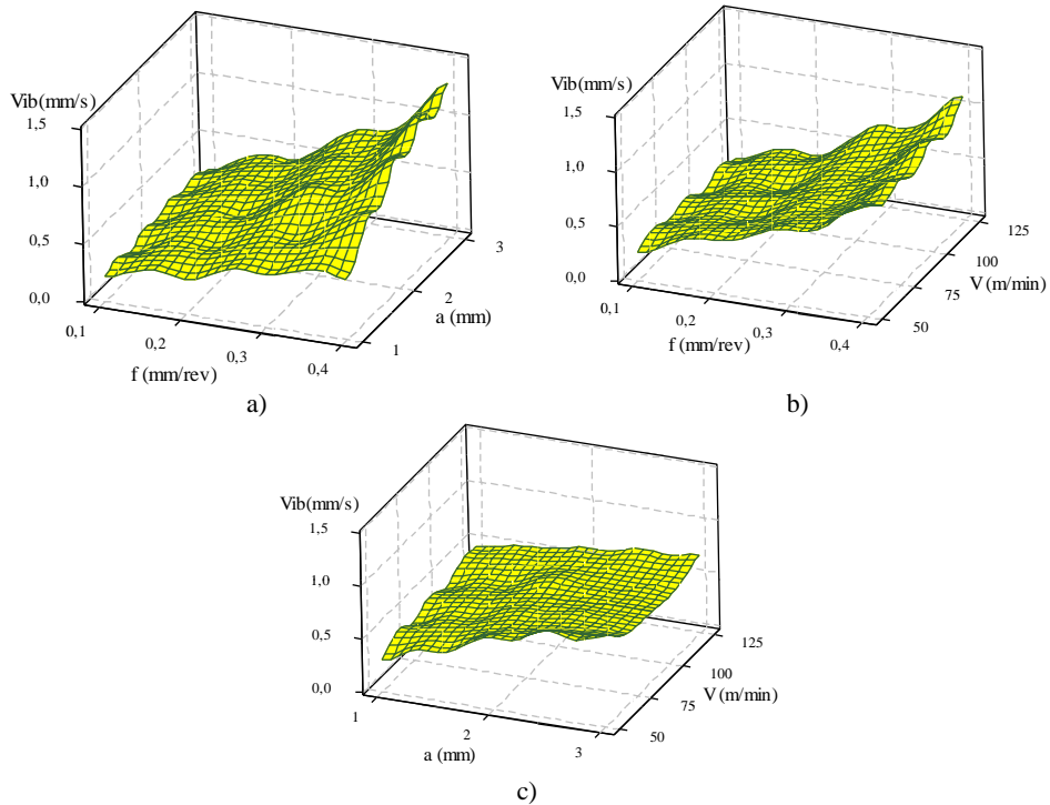
Figure 6. Vibration versus a) feed rate and depth of cut, b) feed rate and cutting speed and c) depth of cut and cutting speed.
