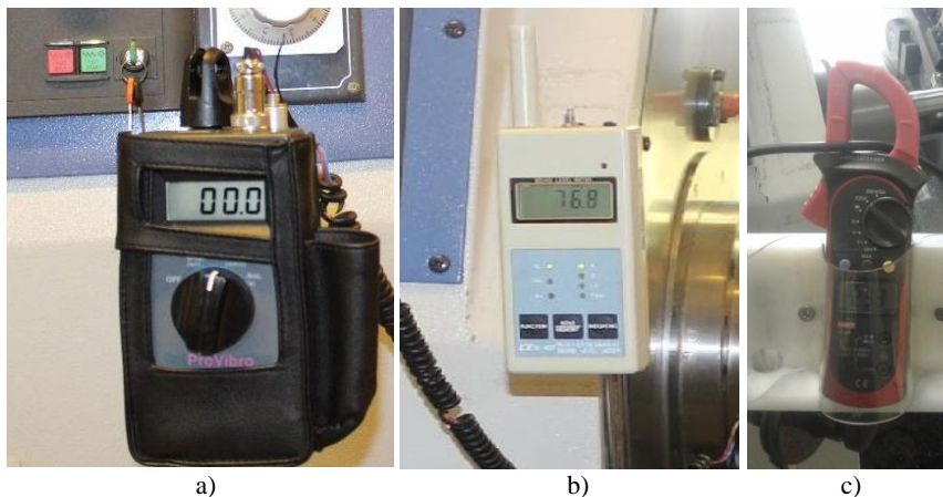
Figure 1. The used devices for measurement of a) vibration, b) sound and c) motor current
