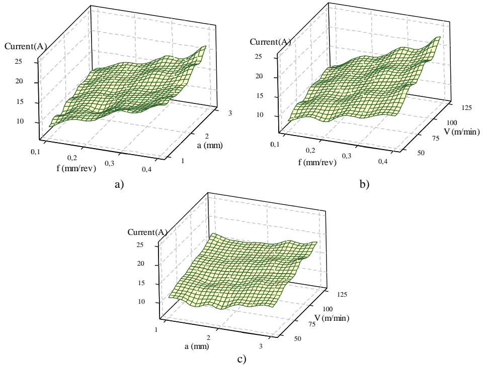
Figure 10. Motor current versus a) feed rate and depth of cut, b) feed rate and cutting speed and c) depth of cut and cutting speed.
