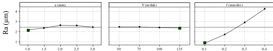
Figure 3. The effect of cutting parameters on means response characteristics for surface roughness.
