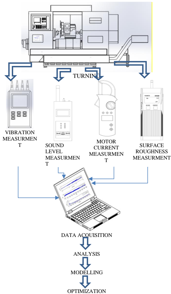
Figure 2. Schematic view of the experimental set-up.
