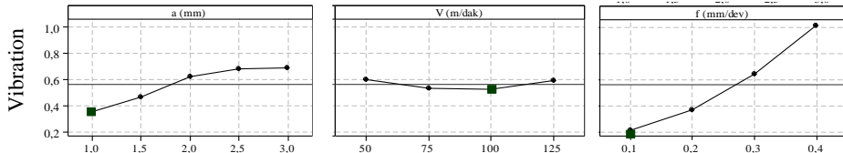
Figure 5. The effect of cutting parameters on means response characteristics for vibration.
