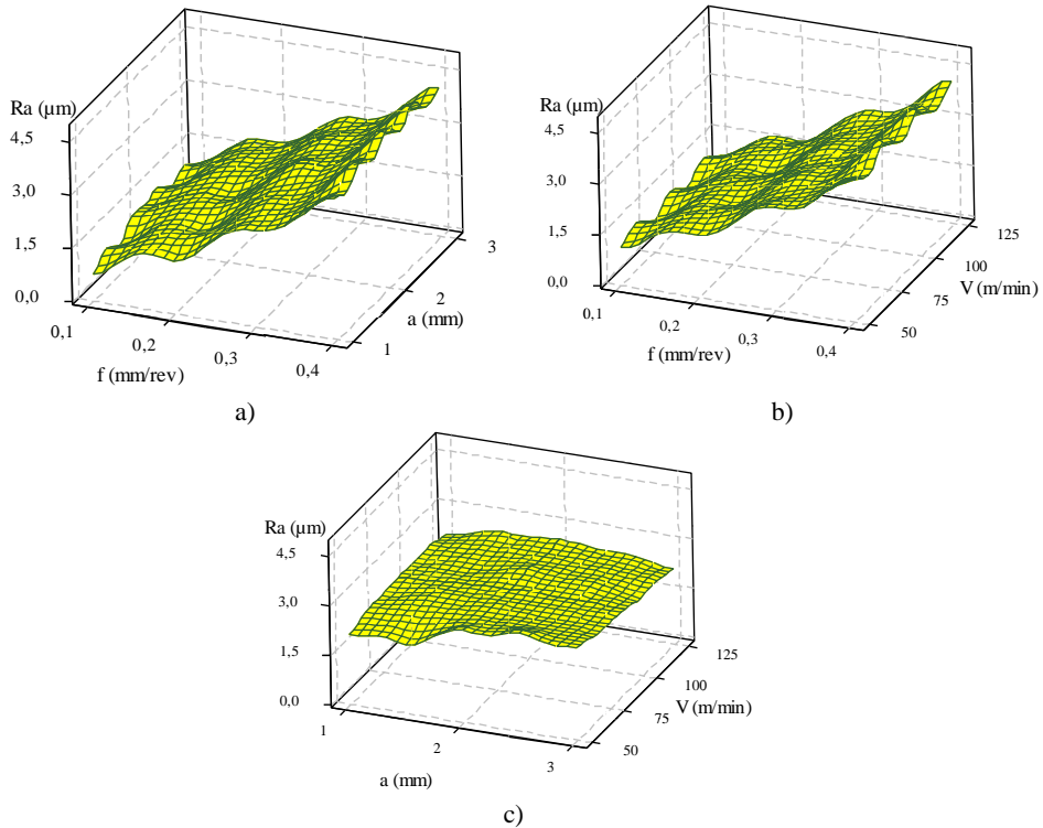
Figure 4. Surface roughness versus a) feed rate and depth of cut, b) feed rate and cutting speed and c) depth of cut and cutting speed.
