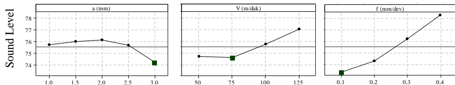
Figure 7. The effect of cutting parameters on means response characteristics for sound level.
