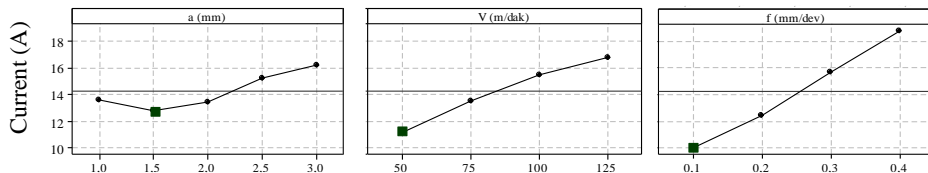
Figure 9. The effect of cutting parameters on means response characteristics for motor current.
