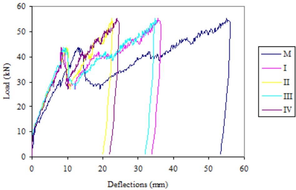
Figure 7. Load Deflection curve of A4 slab
