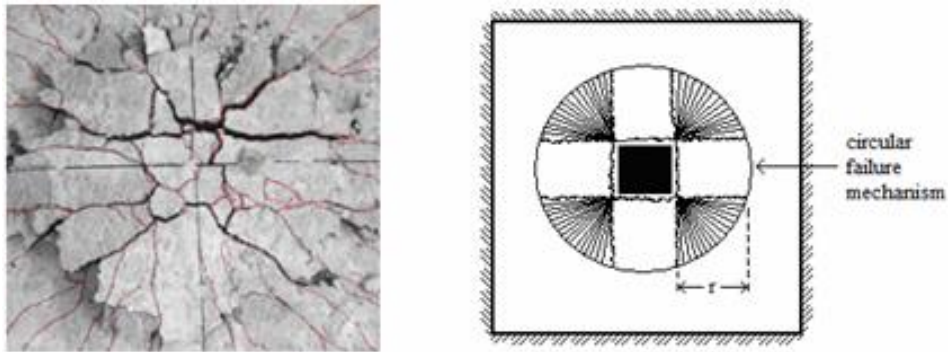
Figure 19. Experimental and theoretical failure mechanisms of a fixed boundary slab
