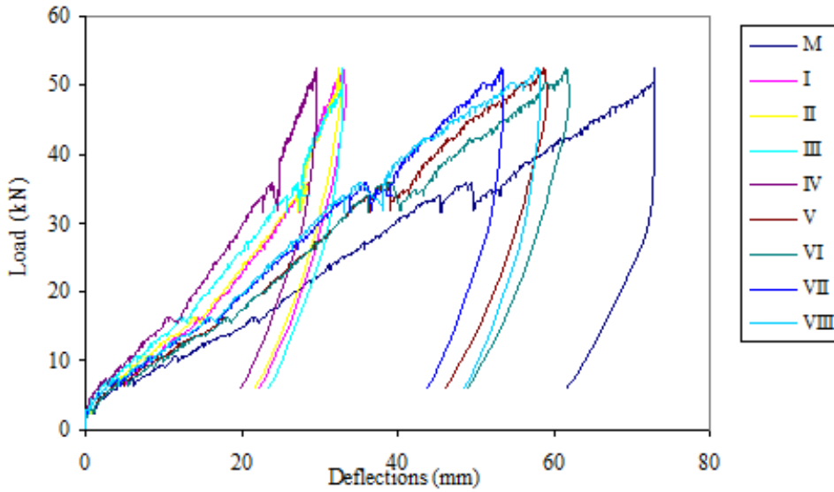
Figure 11. Load Deflection curve of AB4 slab
