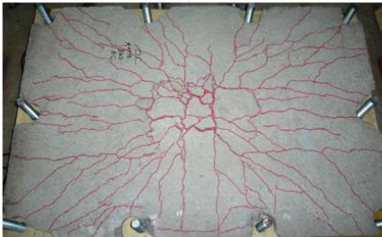
Figure 16. Failure pattern of AGD4 slab
