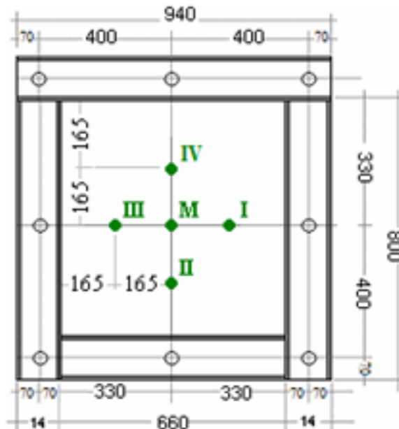
Figure 4. Deflection measurement points for 660x660 mm free-span slabs [16]
