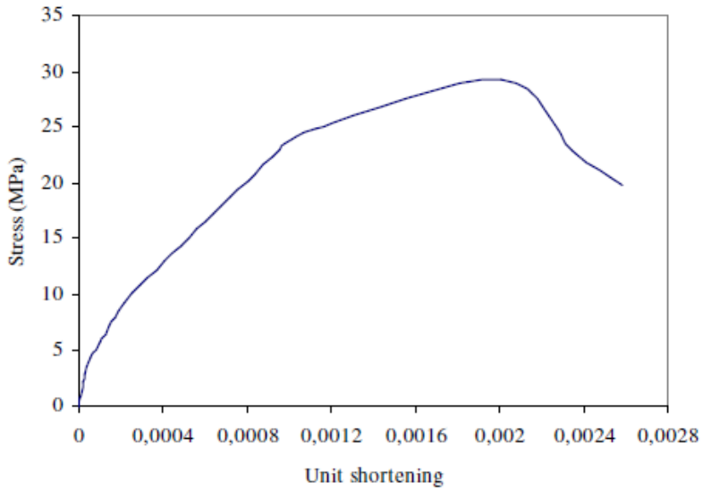
Figure 2. Stress-Strain curve for ordinary concrete
