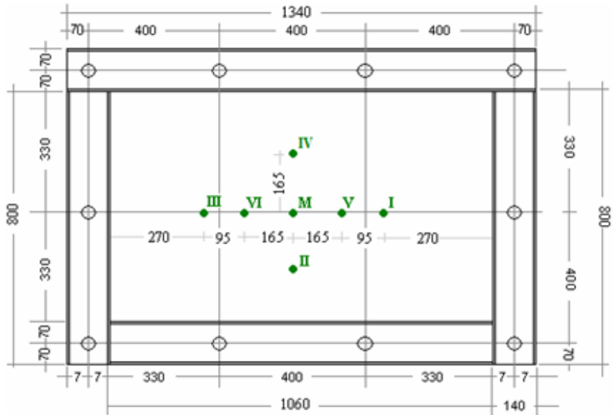
Figure 5. Deflection measurement points for 660x1060 mm free-span slabs [16]
