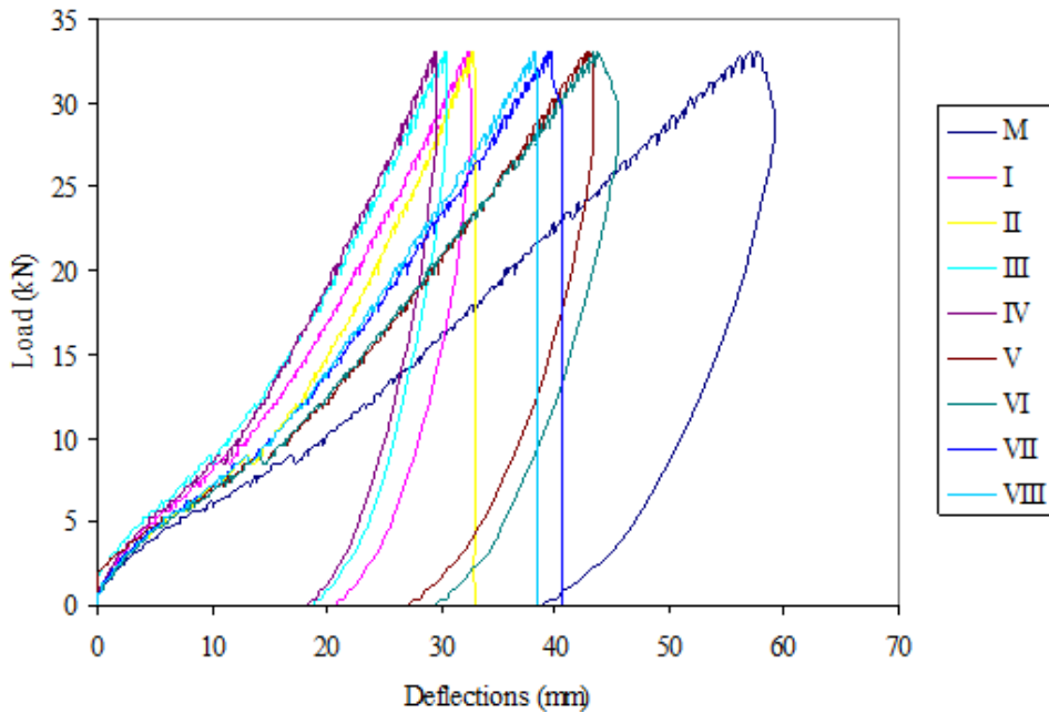
Figure 17. Load Deflection curve of AGB4 slab
