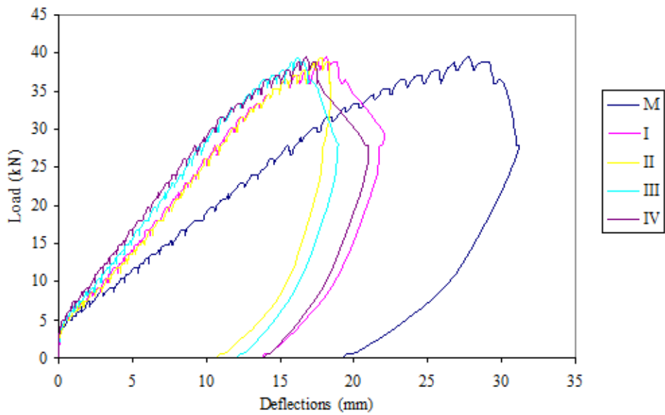
Figure 13. Load Deflection curve of AG4 slab
