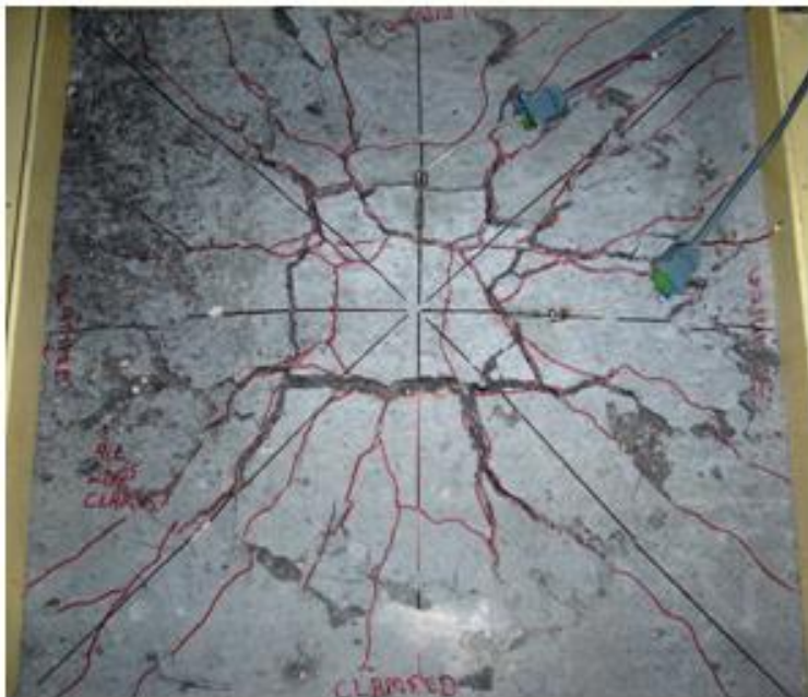
Figure 8. Failure pattern of A4 slab
