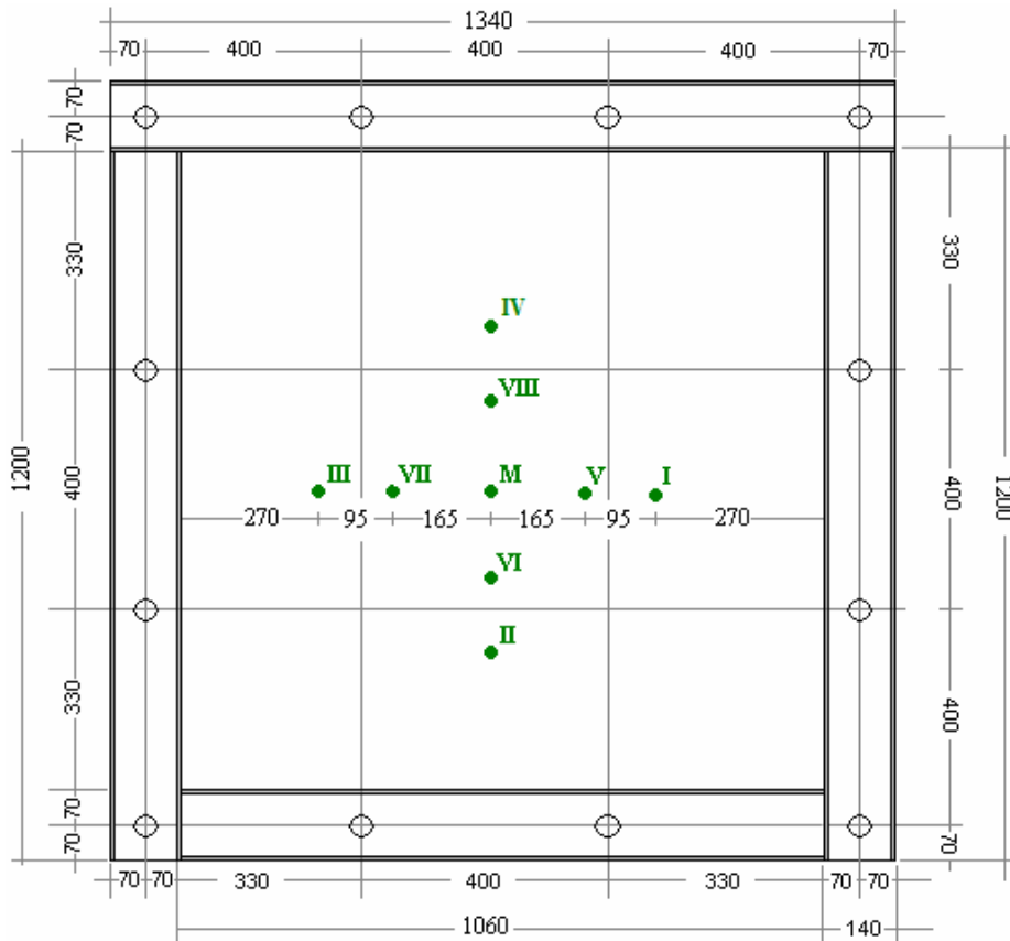
Figure 6. Deflection measurement points for 1060x1060 mm free-span slabs [16]
