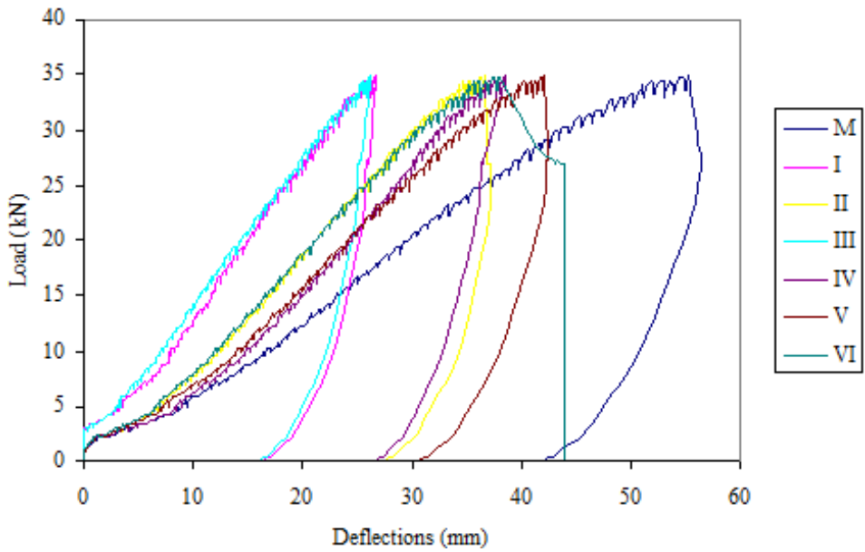
Figure 15. Load Deflection curve of AGD4 slab
