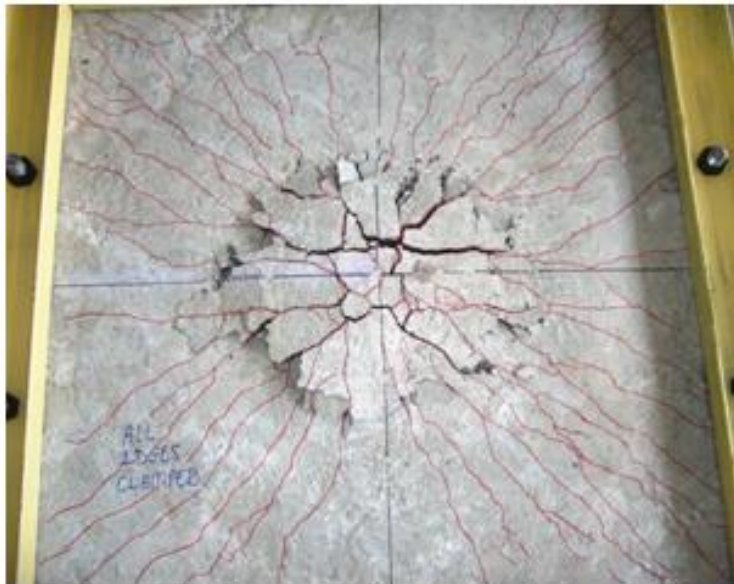
Figure 12. Failure pattern of AB4 slab
