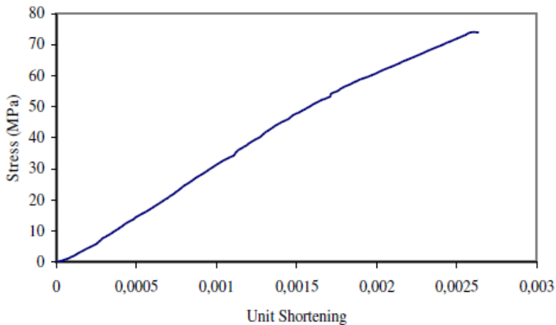
Figure 1. Stress-Strain curve for high-strength concrete
