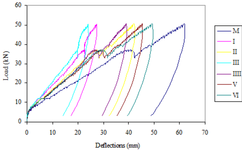
Figure 9. Load Deflection curve of AD4 slab
