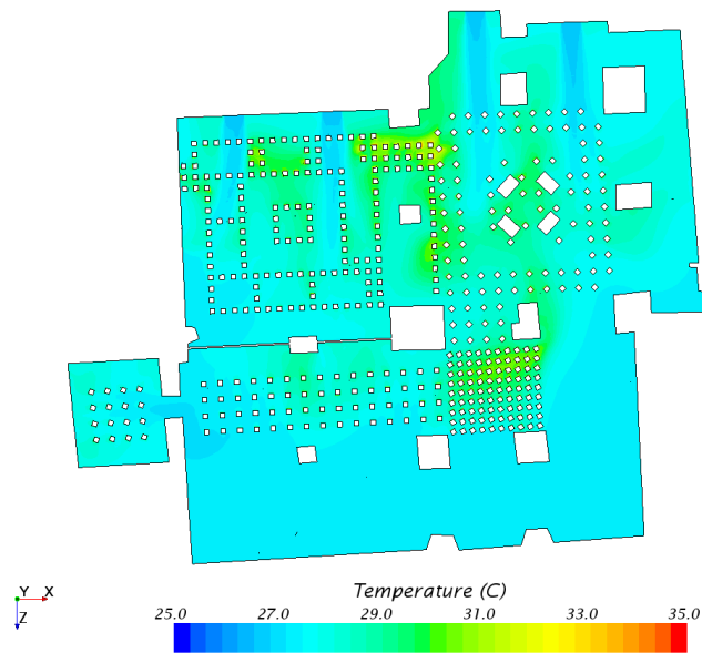
Figure 7: Temperature distribution throughout a horizontal plane located 1.6 m above the floor
