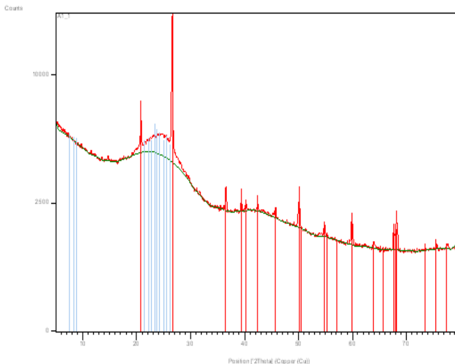
Figure 3. XRD of the activated carbon.
