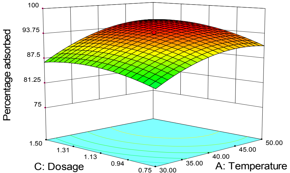
Figure 7. Surface plot between adsorbent dosage and temperature against adsorption efficiency of Pb(II).
