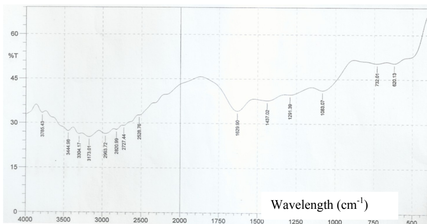
Figure 1. FTIR spectra for the activated carbon (PMAC).
