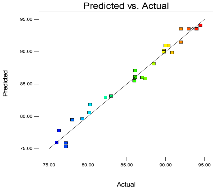
Figure 4. Plot of the predicted adsorption efficiency versus the actual experimental value.
