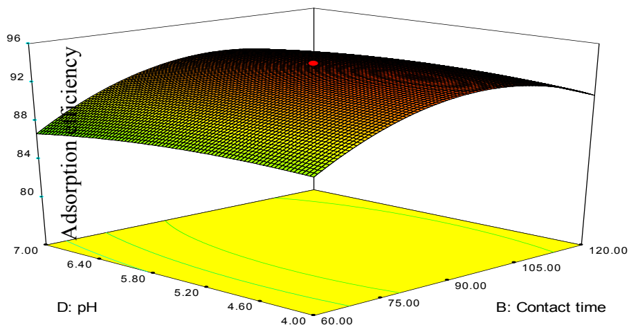
Figure 10. Surface plot between contact time and pH against adsorption efficiency of Pb(II).
