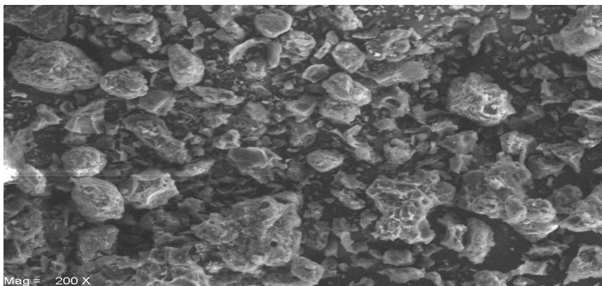
Figure 2. SEM micrograph of PMAC.
