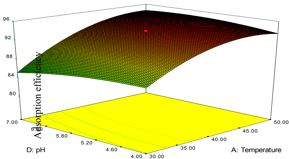
Figure 8. Surface plot between pH and temperature against adsorption efficiency of Pb(II).
