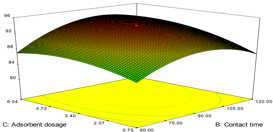
Figure 9. Surface plot between adsorbent dosage and contact time against adsorption efficiency of Pb(II).
