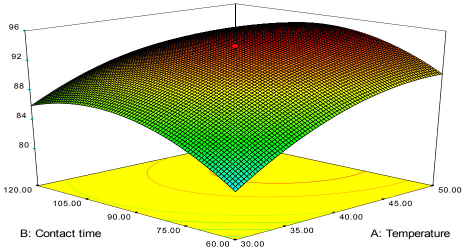
Figure 6. Surface plot between contact time and temperature against adsorption efficiency of Pb(II).
