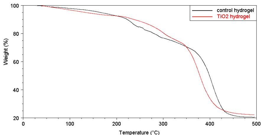
Figure 2. TG curves of hydrogels.
