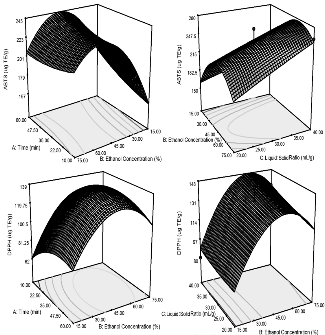
Figure 4. Response surface plots for interactions between the processing variables ABTS + scavenging activity and DPPH scavenging activity.
