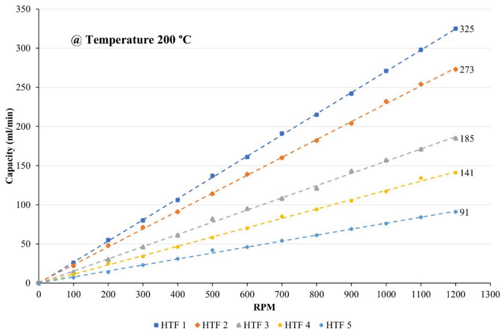
Figure 6. Delivery rate at temperature 200 °C.
