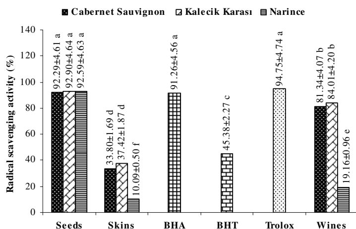
Figure 1-Radical scavenging activities of seeds, skins and wines and standards
