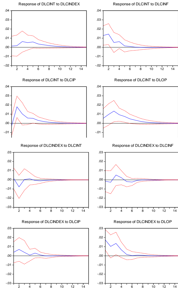
Figure 1: Generalized Responses of Stock Returns of Czech Republic to Shocks in Interest rates, Inflation and Industrial Production and Oil Prices
