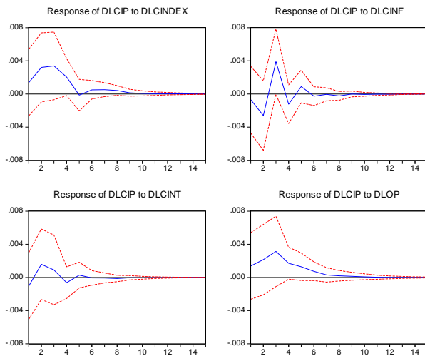
Figure 4: Generalized Responses of Industrial Production of Czech Republic to Shocks in Stock Returns, Inflation, Interest Rates and Oil Prices
