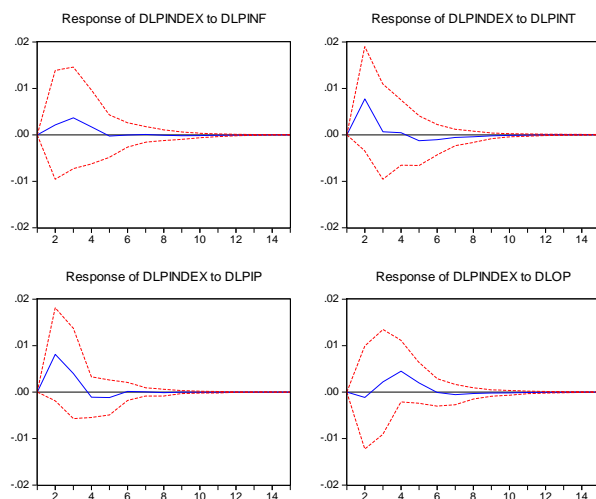
Figure 9: Generalized Responses of Stock Returns of Poland to Shocks in Interest rates, Inflation and Industrial Production and Oil Prices.
