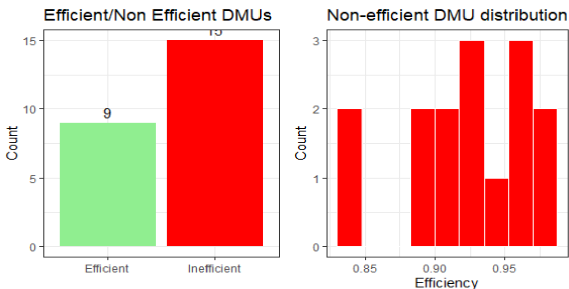
Figure 4. Number of efficient and ineffective countries and efficiency distributions of ineffective countries by CCR model
