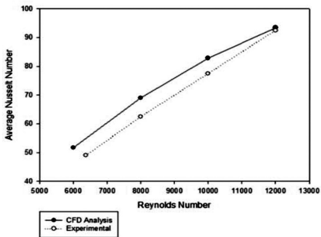
Figure 3. Comparison of numerical and experimental results.
