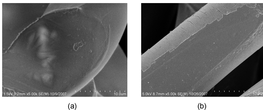
Figure 5. SEM images of the samples' cross sections: (a) original sample; (b) ZnO deposited sample
