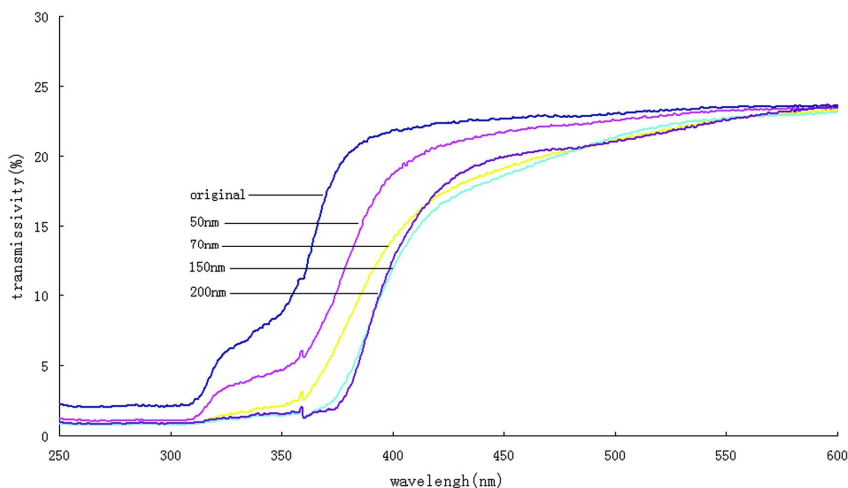
Figure 6. Effect of deposition thickness on the transmittance of the samples
