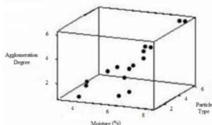
Figure 5. Scatter plot of agglomeration ( \hat{y}_3 ) versus moisture content and particle type
