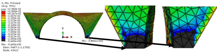
Fig. 12 S_{min} Principal Stress Values Abaqus Analysis Result
