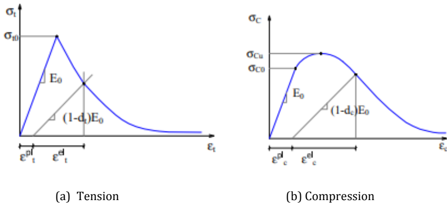
Fig. 4 CDP Tension and Compression Graphs
