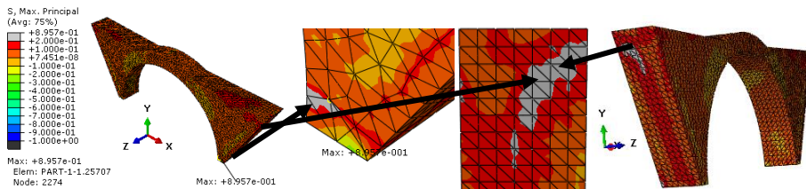
Fig. 11 S_{max} Principal Stress Values Abaqus Analysis Result
