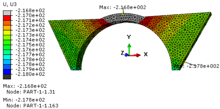
Fig. 10 The Max Displacement at 3.035 s
