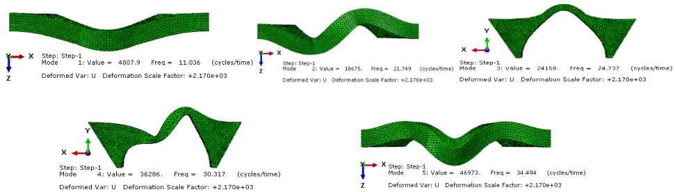
Fig. 8 First 5 Mode and Frequency Values
