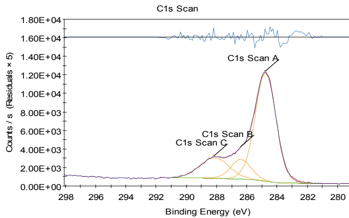
Figure 6. Photoemission spectrums for nitrogen plasma applied to silk fibers (A.O1 s , B.N1 s , C. C1 s ).
