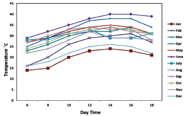
Figure 14. Temperature mapping for month and days high temperature.
