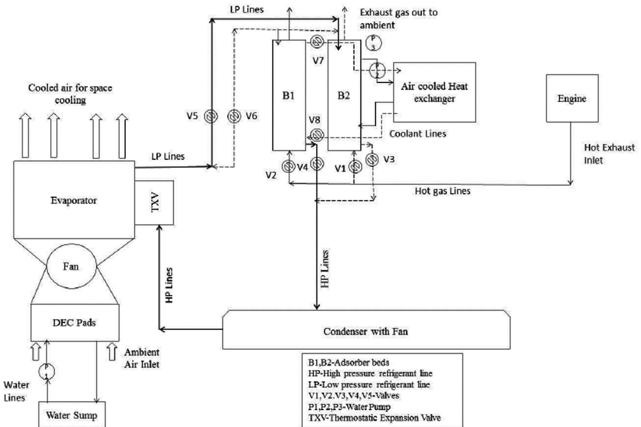
Figure 2. Novel hybrid Air conditioning system.
