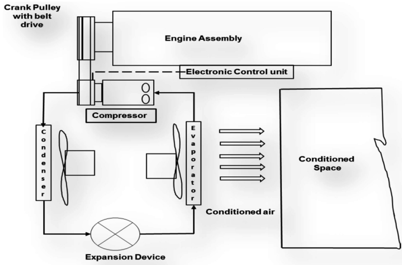
Figure 1. Automobile air conditioning system.
