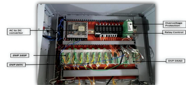
Figure 6. Construction layout of hardware in NMDAS.
