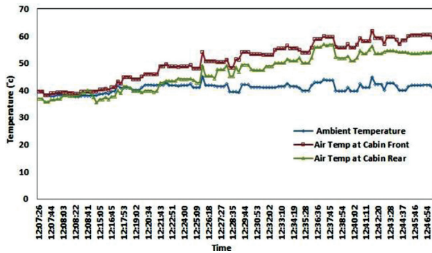
Figure 15. Cabin temperature mapping using NMDAS.
