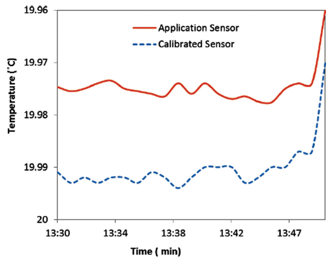
Figure 10. Stability of temperature sensors at 20°C.
