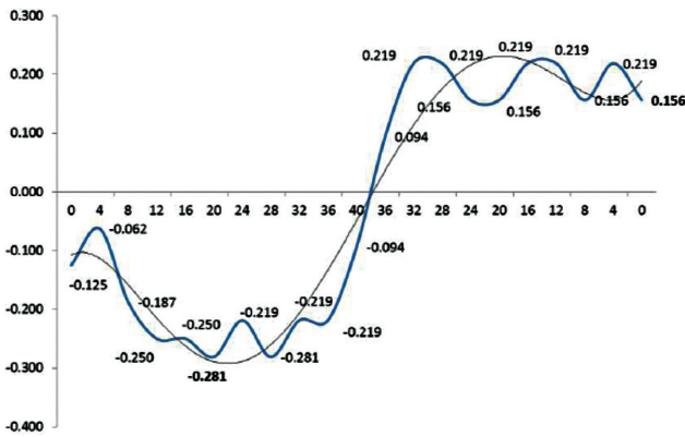
Figure 11. Pressure calibration and error analysis over pressure Span.
