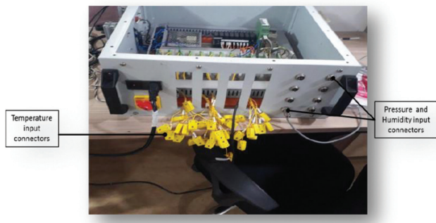
Figure 5. Interfacing of sensors with NMDAS.
