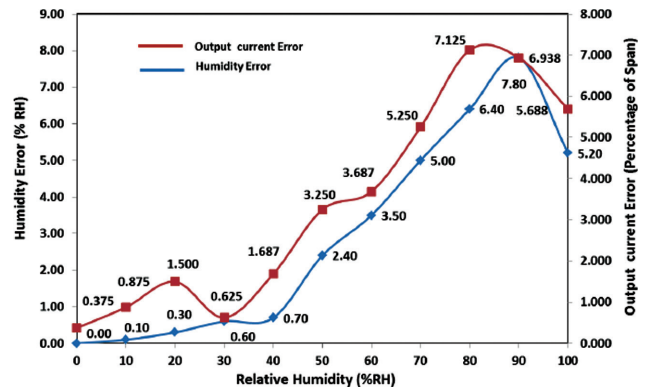
Figure 12. Humidity calibration and error analysis over operating span.
