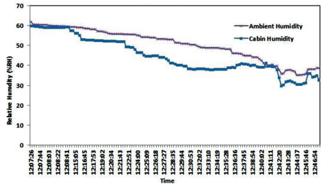
Figure 16. Cabin relative humidity mapping using NMDAS.
