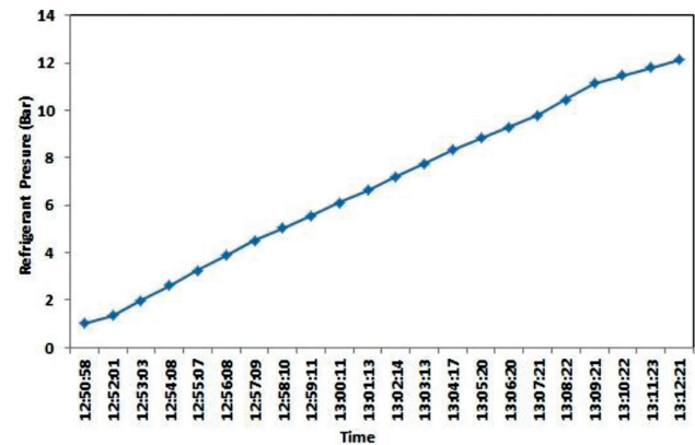
Figure 17. Refrigerant pressure mapping using NMDAS.
