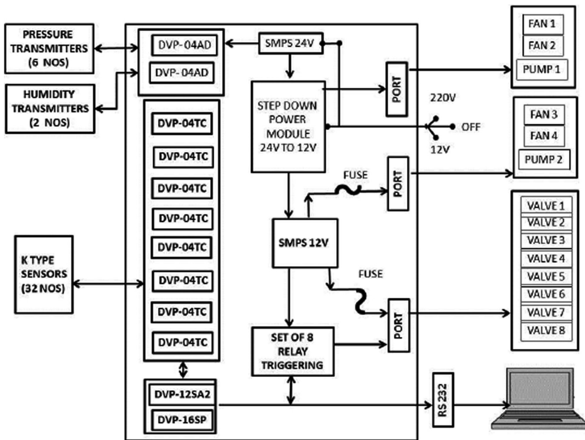
Figure 4. Block diagram of NMDAS.
