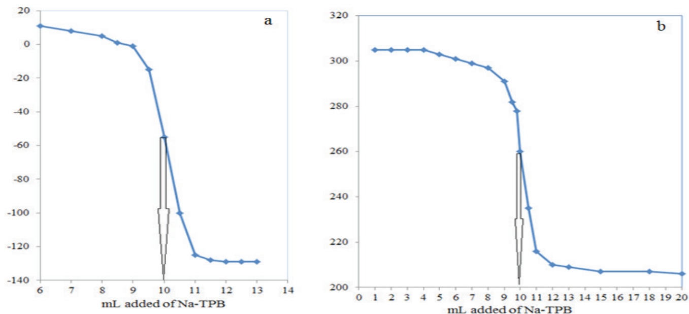
Figure 5. Potentiometric titration of 10 mL of 1.0 \times 10^{-3} mol/mL HP with 1.0 \times 10^{-3} mc Na-TPB using (a) sensor P and (b) sensor g
