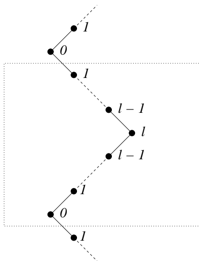
FIGURE 6. A full heap, \overline{E} , over the Dynkin diagram of type C_l^{(1)} (l > 1)
