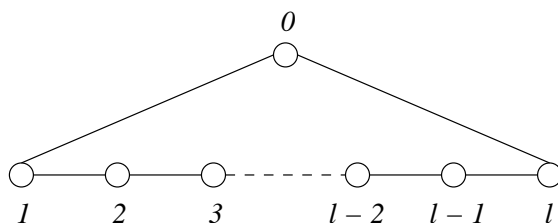
FIGURE 3. The Dynkin diagram of type A_l^{(1)} (l > 1)
