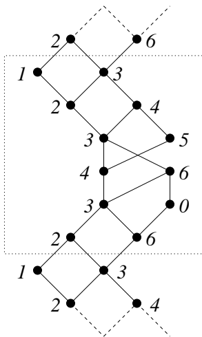
FIGURE 16. A full heap over the Dynkin diagram of type E_6^{(1)}
