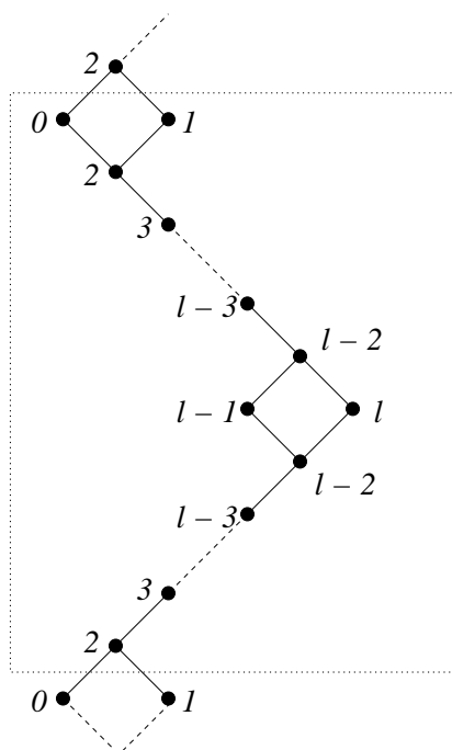
FIGURE 9. A full heap, E , over the Dynkin diagram of type D_l^{(1)}
