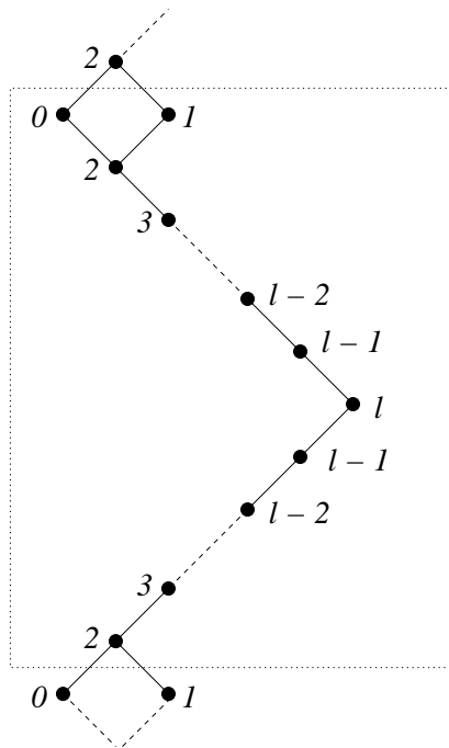
FIGURE 11. A full heap, \bar{E} , over the Dynkin diagram of type A_{2l-1}^{(2)}
