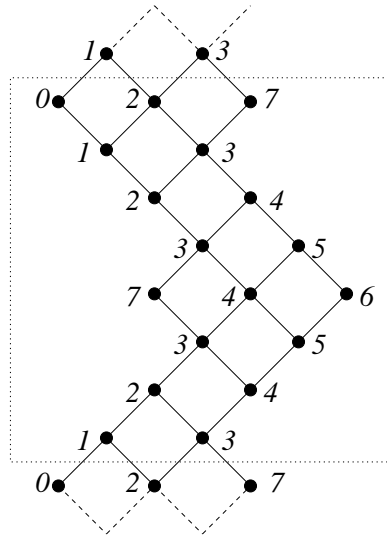
FIGURE 18. A full heap over the Dynkin diagram of type E_7^{(1)}
