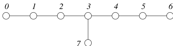
FIGURE 17. The Dynkin diagram of type E_7^{(1)}
