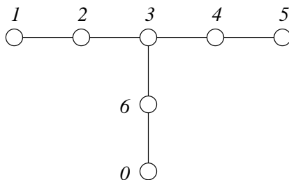
FIGURE 15. The Dynkin diagram of type E_6^{(1)}
