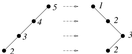
FIGURE 2. The heaps F and \bar{F} of Example 6.4
