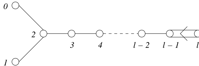
FIGURE 10. The Dynkin diagram of type A_{2l-1}^{(2)}
