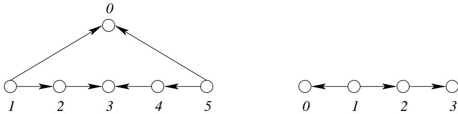
FIGURE 1. Compatible orientations for the Dynkin diagrams of types A_5^{(1)} and C_3^{(1)} in Example 6.4
