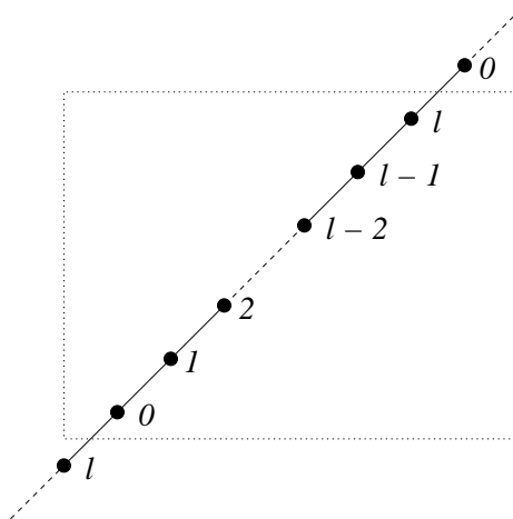
FIGURE 4. A full heap, E , over the Dynkin diagram of type A_l^{(1)} (l > 1)
