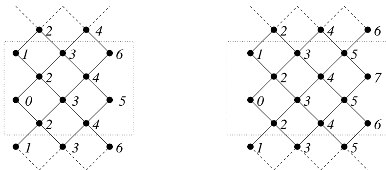
FIGURE 12. Full heaps over the Dynkin diagram of type D_l^{(1)} for l = 6 and l = 7
