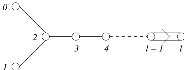
FIGURE 13. The Dynkin diagram of type B_l^{(1)}
