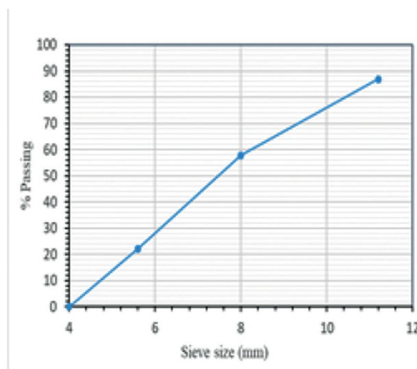
b) Particle size distribution of NO I RCA
