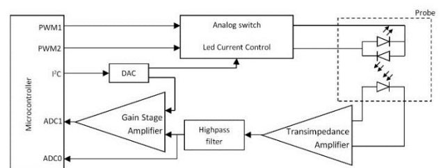
Figure 8: Block diagram of pulse oximeter.
