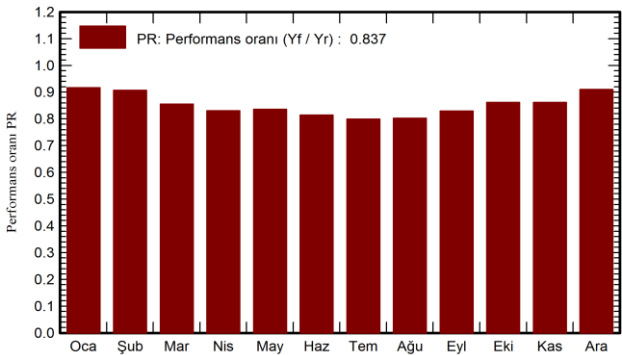
Şekil 3.6 25° Polikristal panelli sistemin yıllık ortalama performans oranı (Figure 3.5 Average annual performance rate of system 25° orientation angle Polycrystalline panel)
