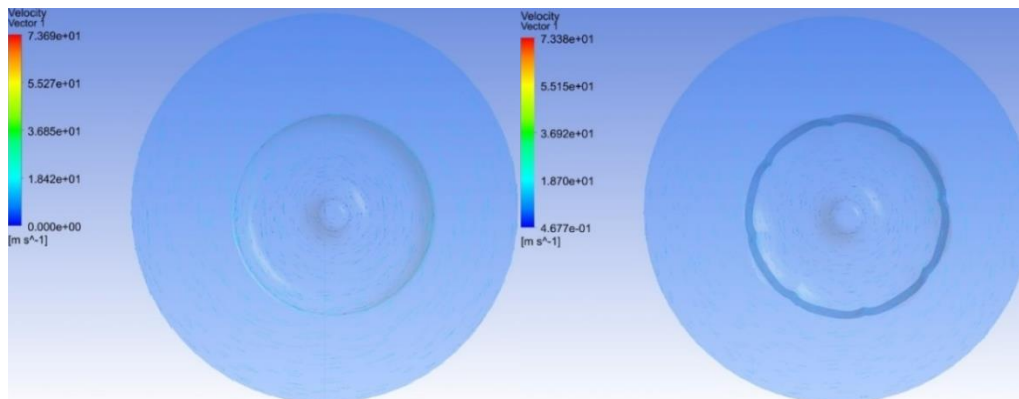
Fig. 6. Fluid velocity distribution in the x-y plane before TDC (692° CA)
