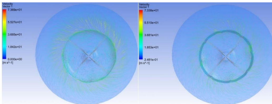
Fig. 7. Fluid velocity distribution in the x-y plane in TDC (720° CA)
