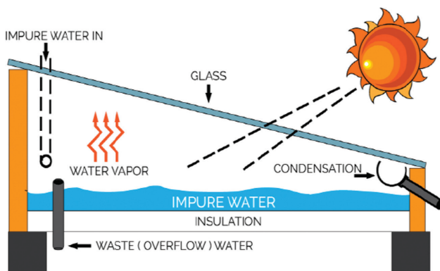
Figure 10. Single slope solar distillation unit.
