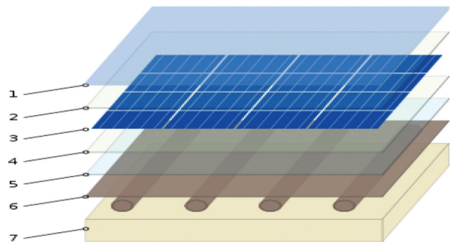
Figure 17. Cross sectional view of PVT (1. Anti reflective glass, 2. Encapsulant, 3. Solar PV cells, 4. Encapsulant, 5. Backsheet, 6. Heat exchanger, 7. Thermal insulation).
