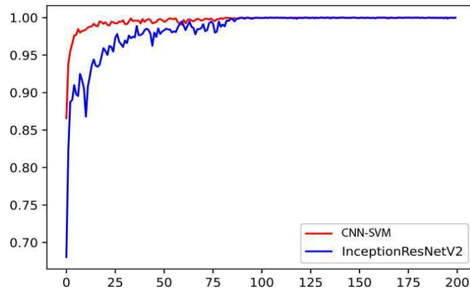
Figure 5. CNN-SVM vs RESnet Accuracy
