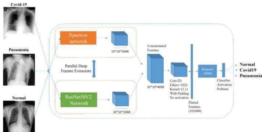
Figure 3. Proposed Network detection
