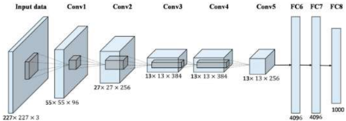
Figure 1: AlexNet Structure
