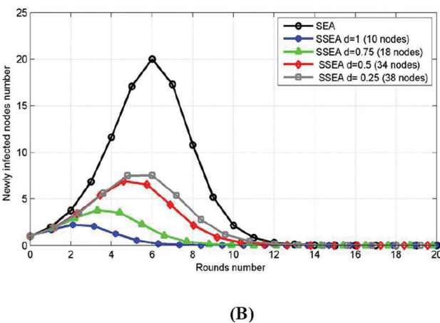
Figure 6. Total infected nodes in SSEA for selection of nodes with specific d values.
