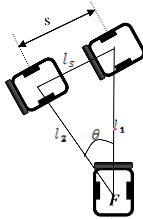
Fig. 6. Second way of calculation of the average speed of enemy.
