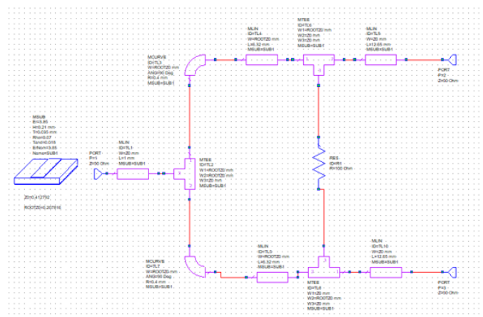
Figure 3. Two Way Power Divider Circuit Schematic
