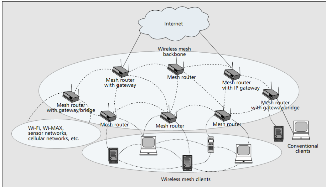
Fig. 2: Hybrid WMN.
