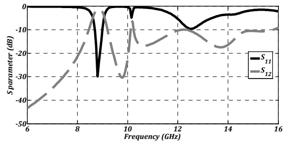
Figure 2. Return loss and insertion loss of the bandpass filter
