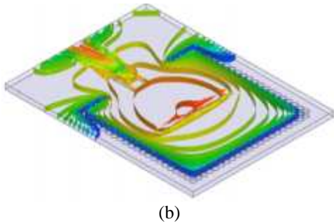
Figure 3. Contour map for the electric field distribution in the two cavities a)top layer b)bottom layer
