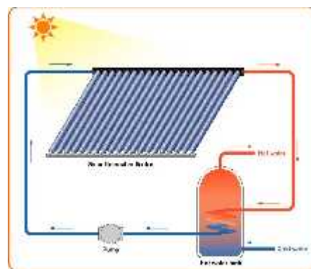
Figure 5. Solar-Powered Hot Water Supply System Analysis [7]
