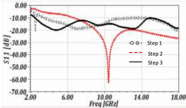
Fig. 2. Three supplementary antenna designing steps
